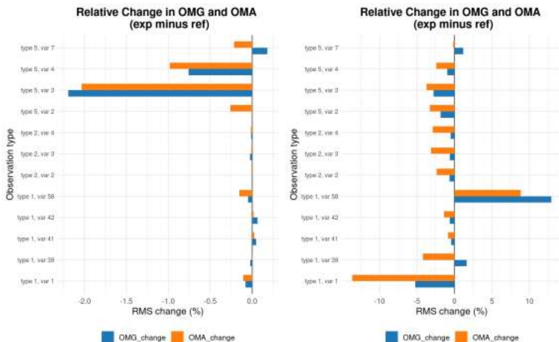
Figure 6.1.1: (left) Impact of 3DEnVar perturbations as two sub-ensembles in Cleaf1k on departure statistics, (right) Impact of scale-dependent localization (SDL). Negative values indicate improvement with respect to the reference. Validation period is 1 month in winter 2025.
