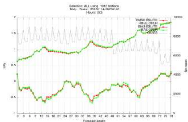
Figure 2.2.1: Changes of the scores in ALADIN/SHMU, between reference (63L) and esuite (87L) for MSLP.
