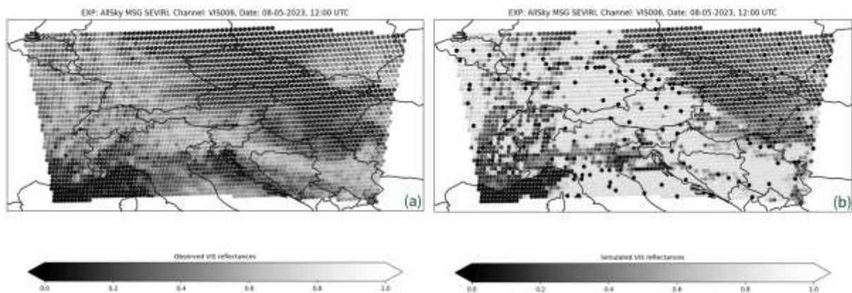
Figure 3.2.3: Visible channel 0.6um, Observation(left) and Simulation(right) from MSG SEVIRI.
