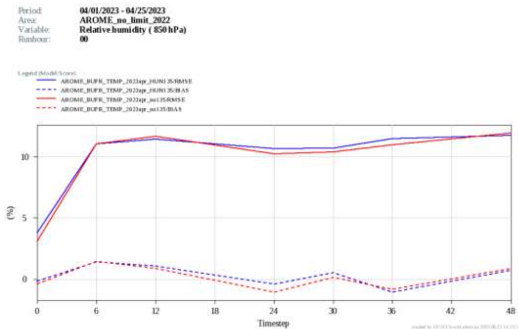
Figure 1.1.1: Bias (dashed line) and RMSE (solid line) of relative humidity forecasts at 850 hPa as a function of lead time for AROME experiments using BUFR TEMP data with (blue) and without (red)
