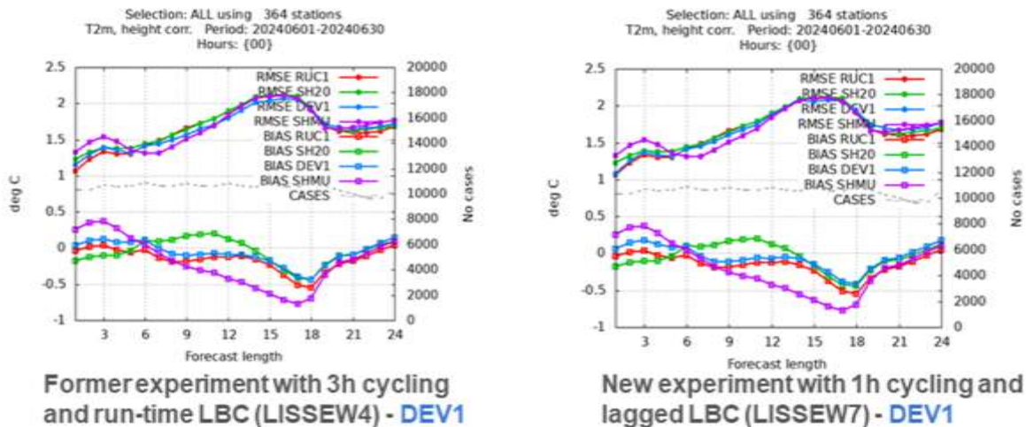
Figure su1.5: Scores from the “dev” experiments with smoothing the deep soil wetness in 1km resolution rapid update cycle for the 1 month period of June 2024.
