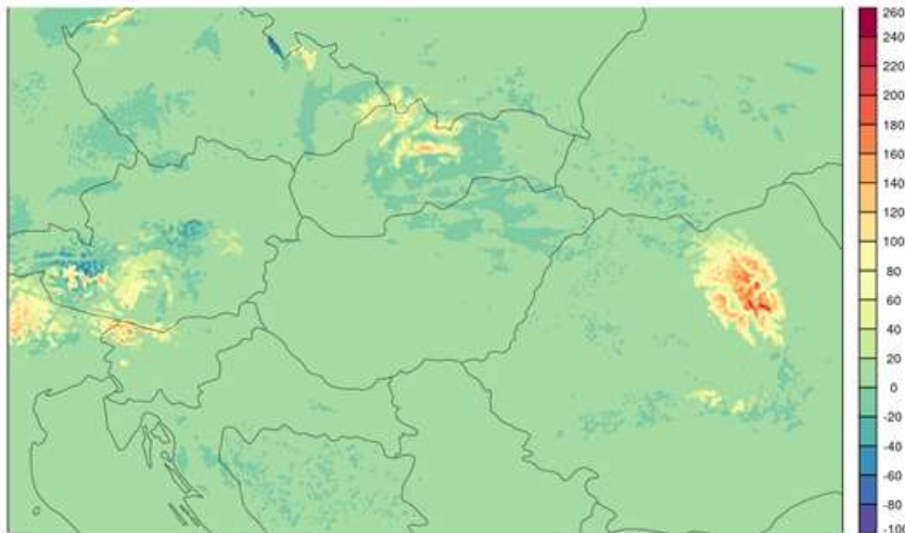
Figure su1.3: The difference of the snow-water equivalent [ \text{kg}/\text{m}^2 ] between experiment with the modifications and the reference run at 6 UTC on 2 February 2025.
