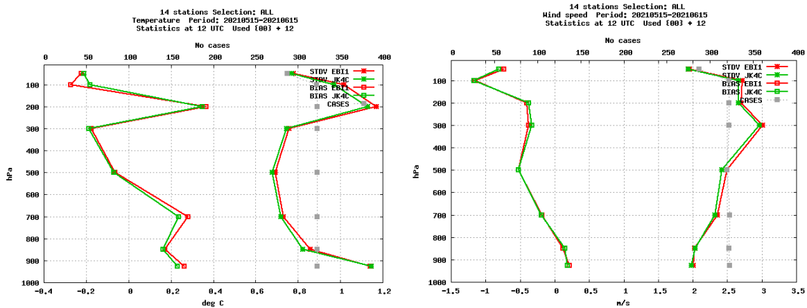
Figure 1.2: Comparison of reference (no Jk; red) and Jk (with Jk; green) experiments for temperature (left) and wind speed (right) for +12 forecast range.
