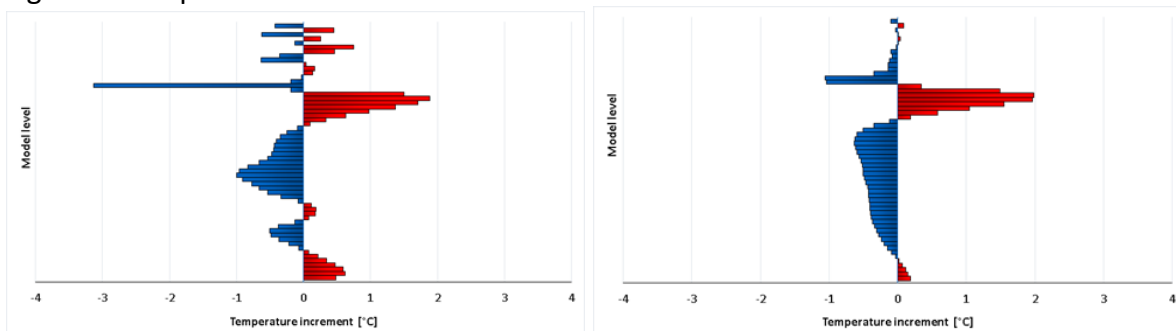
Figure 4.1: Analysis increments with radiosonde data at 6 UTC on 12 December 2021 (left) and without it (right) in the function of model levels.
