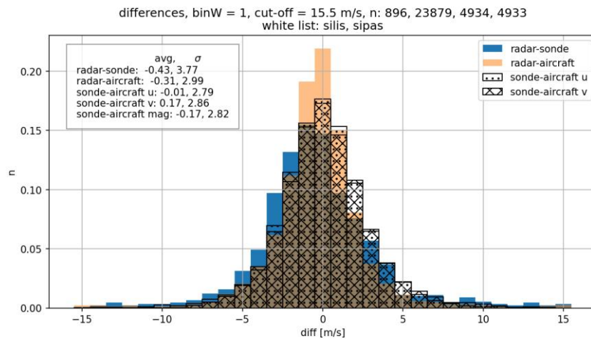
Figure 3.1: The distribution of differences between pairs of colocated radar, radiosonde and aircraft observations (all calculated in terms of Doppler radial wind) for countries with high NI (top), for those with NI < 30 m/s (middle) and for the Slovenian two radars (bottom).
