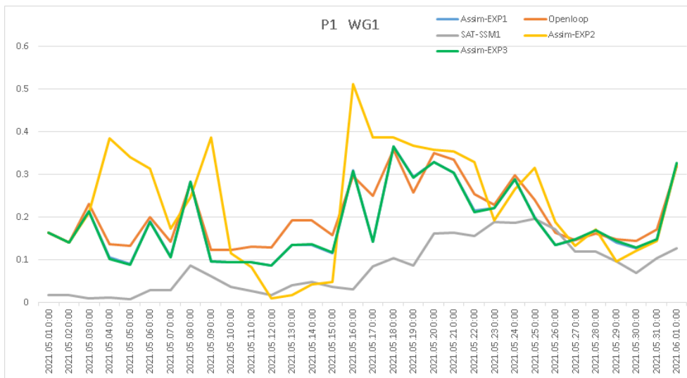
Figure S2.1: Satellite superficial soil moisture observations along with an open loop SURFEX run and various data assimilation experiments for a point near Budapest for a period of one month.
