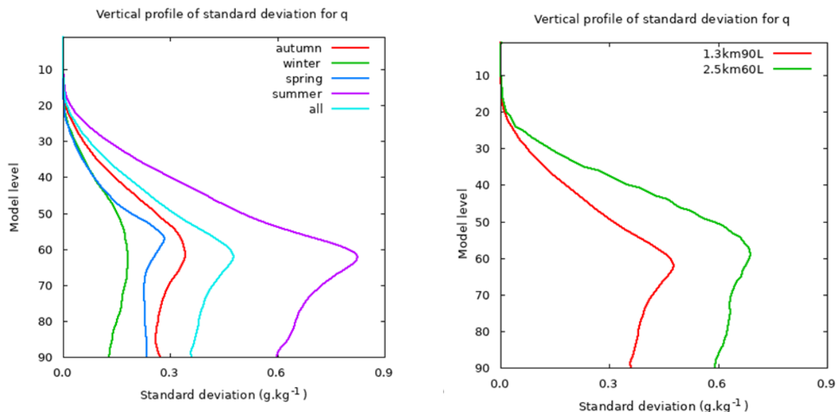
Figure 1.1: Vertical profiles of standard deviation for humidity in the downscaled B-matrix at 90 levels in the four seasons all together and separately (left) and in the previously computed B-matrix at 60 levels and the downscaled B-matrix at 90 levels (right). [registered under COM3.1]
