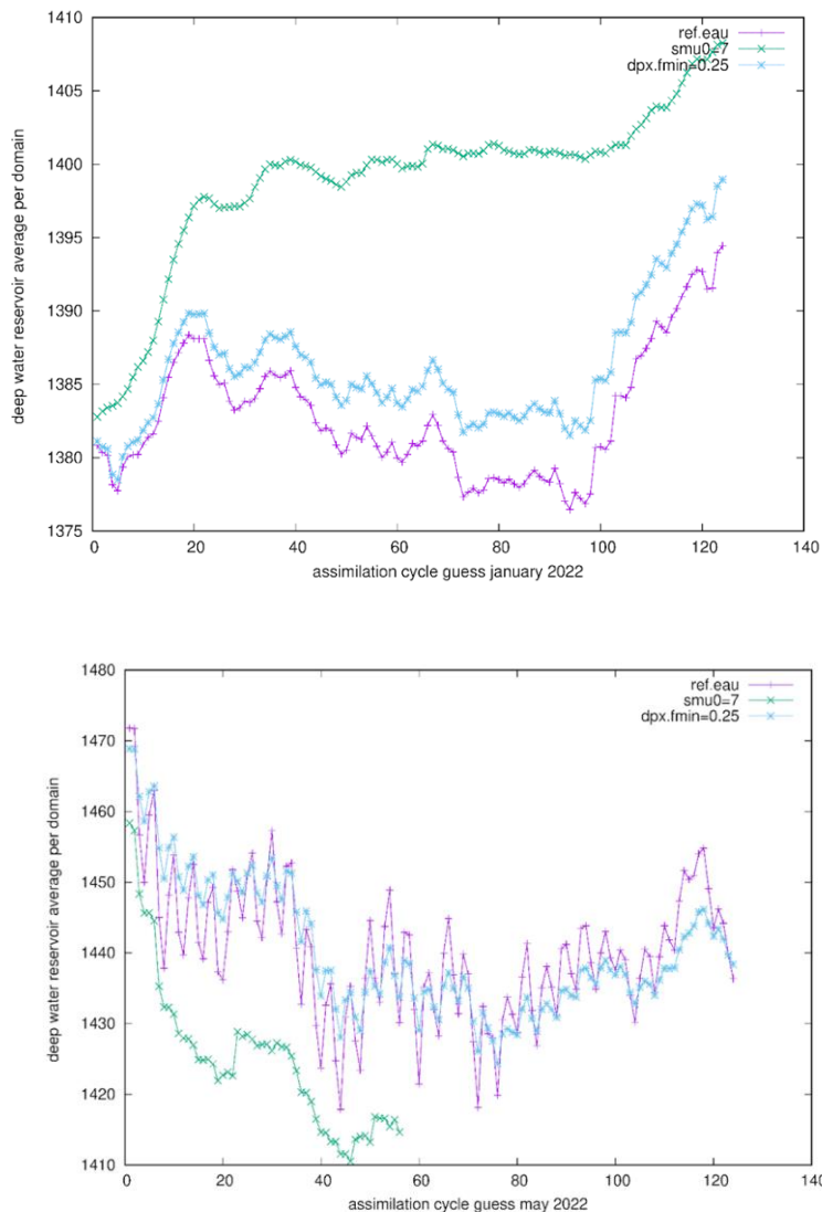
Figure S1.2: The evolution of the horizontal average of deep soil water reservoir during the assimilation cycle. The examples are from January and May 2022. In reference the deep soil water increment is not diminished, which in summer causes diurnal oscillations. When the modulation increments by solar zenith angle is applied setting SMU0=7 , we remove diurnal
