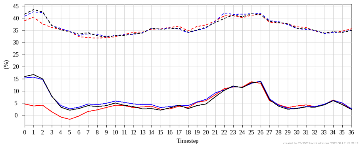
Figure 3.3: Bias (solid line) and RMSE (dashed line) of total cloudiness in function of the lead time for the 0 UTC runs of the test experiment (red), the reference run (blue) and the operational AROME (black).
