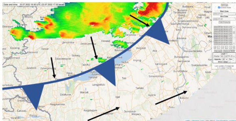
2km CAPPI radar reflectivity [dBz] and schematics of the cold front position and flow on 23 July 2022 15 UTC after observations
