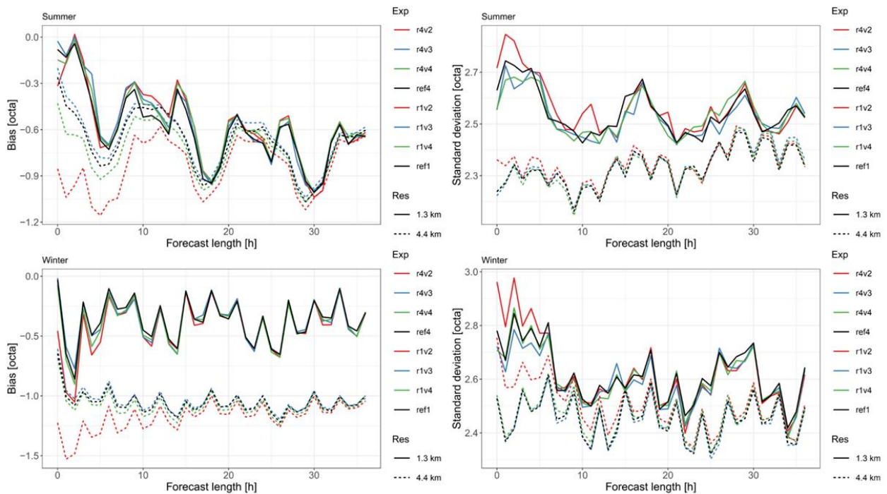
Figure 3.2: Bias (left) and standard deviation (right) of cloudiness for summer and winter period in ALARO suites at 1.3 (full line) and 4.4 km (dashed line). Reference experiment (black), default radar DA in red, wet-pixels only experiment (green) and modified drying using the non-rainy environment (blue). The default radar reflectivity DA setup clearly degrades the cloudiness while the alternative approaches perform clearly better.
