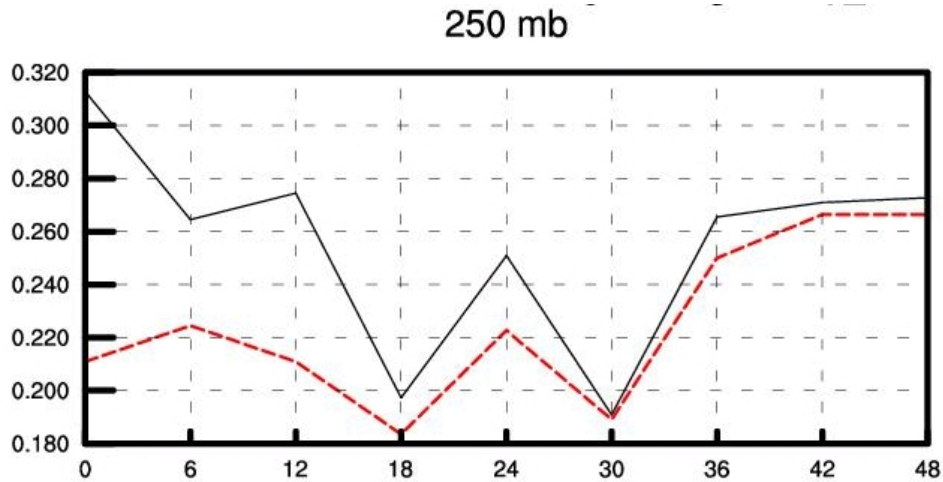
Figure 10: Root mean square forecast errors of relative humidity (in percent) at 250 hPa level against radiosonde observation. Comparison of two 3D-Var runs with ATOVS data assimilated in 80 km resolution. Solid line: when the multivariate formulation was used for all control variables ( T800 ). Dashed line: when the specific humidity was assimilated in univariate form ( touhu ). X axis presents the forecast ranges in hour.
