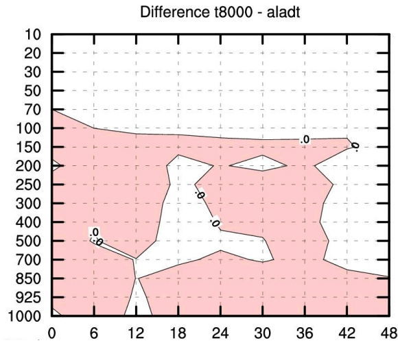
Figure 7: Difference between the root mean square errors for geopotential height: RMSE_{T8000} - RMSE_{Aladt} . Negative value (coloured) means that the error of run with ATOVS data is less than that of control run, thus the ATOVS data have positive impact. X and Y axes present the forecast ranges and the model levels respectively.
