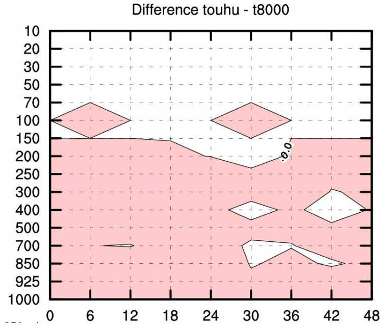
Figure 9: Difference between the root mean square errors of relative humidity: RMSE_{Touhu} - RMSE_{T8000} . Negative value (coloured) means that the error is reduced when assimilating the specific humidity in univariate form.
