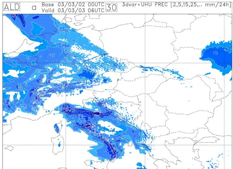
Figure 16: The 24 hour cumulative precipitation (in mm) predicted over the ALADIN/HU domain from 2003.03.02 00 UTC. Upper picture: control run (with TEMP and SYNOP). Lower picture: 3D-Var run with ATOVS assimilated in 80 km resolution. In both runs the humidity was assimilated in univariate form. Note that the 24 hour cumulated precipitation is the difference between the cumulative precipitation predicted at 6 and 30 hour forecast ranges.
