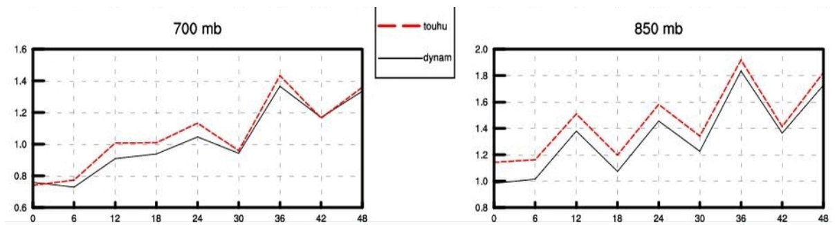
Figure 14: Root mean square forecast errors of temperature (in Kelvin) at 700 and 850 hPa model levels. Comparison of scores of a dynamical adaptation ( dynam , solid line) and a 3D-Var with ATOVS data assimilated in 80 km resolution ( touhu , dashed line). X axis presents the forecast ranges in hour.
