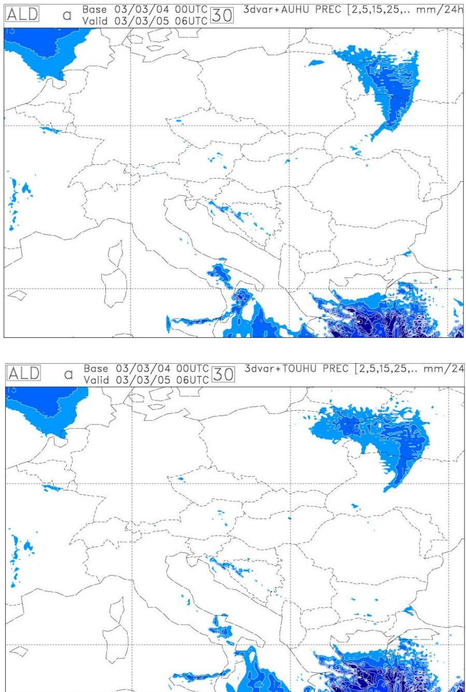
Figure 18: The 24 hour cumulative precipitation (in mm) predicted over the ALADIN/HU domain from 2003.03.04 00 UTC. Upper picture: control run (with TEMP and SYNOP). Lower picture: 3D-Var run with ATOVS assimilated in 80 km resolution. In both runs the humidity was assimilated in univariate form. Note that the 24 hour cumulated precipitation is the difference between the cumulated precipitation predicted at 6 and 30 hour forecast ranges.
