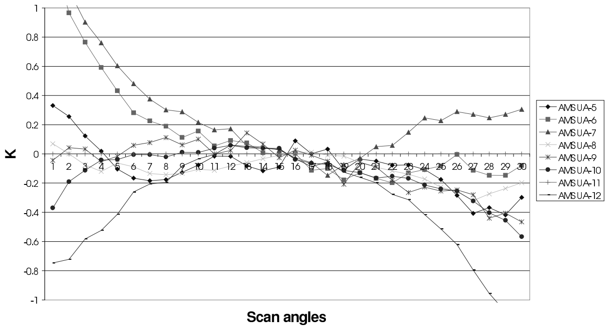
Figure 2: Bias (in Kelvin degree) specific to the scan angles varies with latitude band. In these figures biases were computed for the same latitude band.
