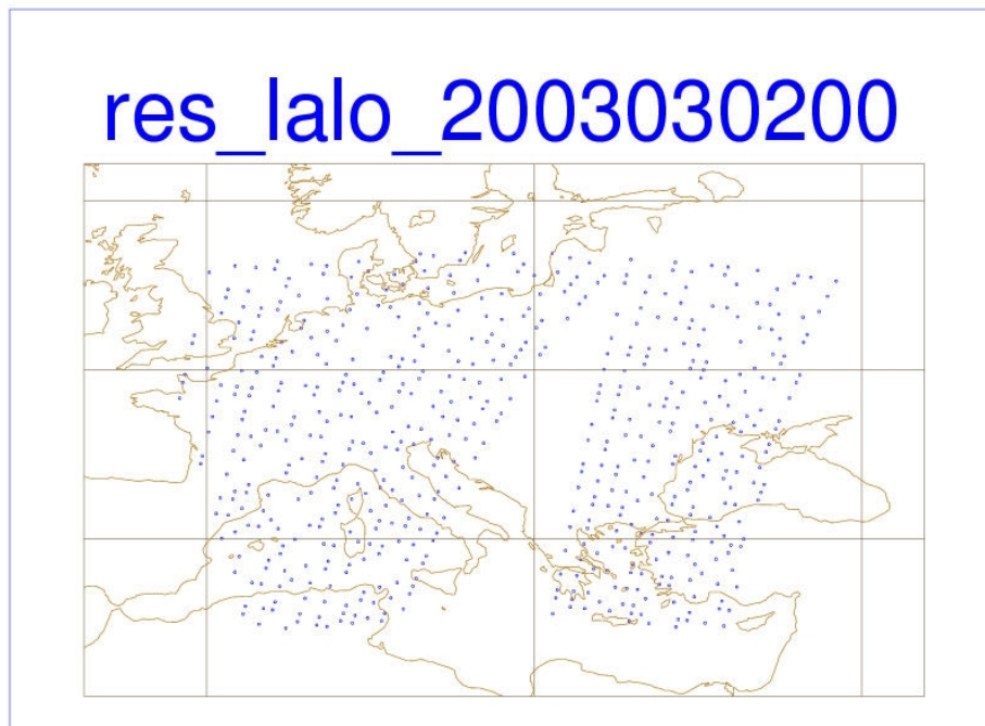
Figure 17: The 24 hour cumulative precipitation (in mm) extracted from SYNOP telegrams for 2003.03.03 06 UTC (upper picture) and the distribution of the ATOVS pixels 2003.03.02 00 UTC (situation after screening - active observation) (lower picture).
