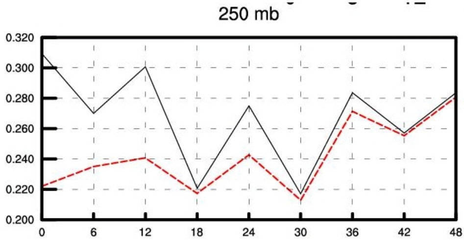
Figure 11: Root mean square forecast errors of relative humidity (in percent) at 250 hPa level against radiosonde observation. Comparison of two 3D-Var runs with TEMP and SYNOP data. Solid line: when the multivariate formulation was used for all control variables ( aladt ). Dashed line: when the specific humidity was assimilated in univariate form ( aluhu , dashed line). X axis presents the forecast ranges in hour.
