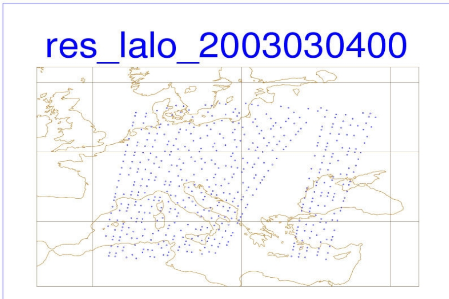
Figure 19: The 24 hour cumulative precipitation (in mm) extracted from SYNOP telegrams for 2003.03.05 06 UTC (upper picture) and the distribution of the ATOVS pixels at 2003.03.04 00 UTC (situation after screening - active observation) (lower picture).
