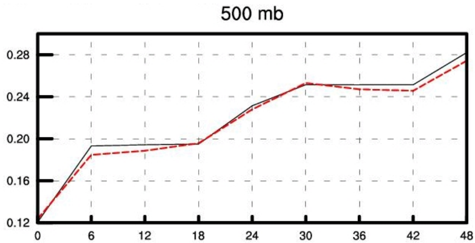
Figure 12: Root mean square forecast errors of relative humidity (in percent) at 500 hPa level against radiosonde observation. Comparison of two 3D-Var runs with ATOVS data when the humidity was assimilated in univariate form. Dashed line: thinning in 80 km ( touhu ). Solid line: thinning in 120 km ( 120uhu ). X axis presents the forecast ranges in hour.
