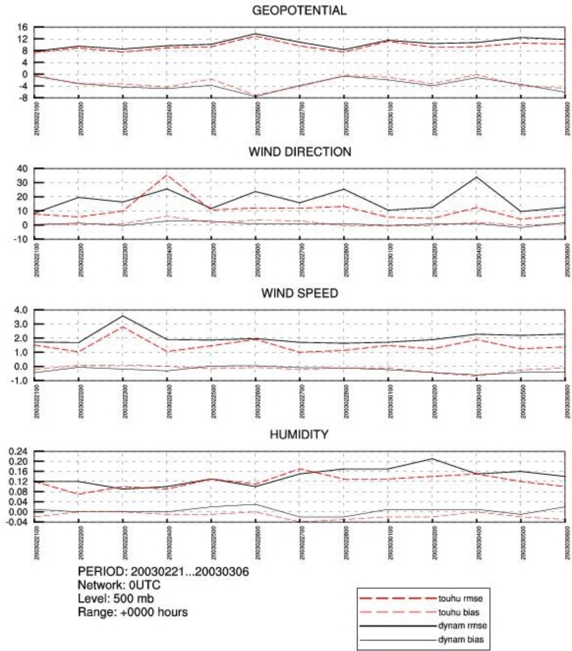
Figure 13: Comparison of day-to-day statistics (RMSE - upper curves and bias - lower curves) of dynamical adaptation run ( dynam , solid line) and 3D-Var run with ATOVS data assimilated in 80 km resolution ( touhu , dashed line). The statistics correspond to 500 hPa model level.
