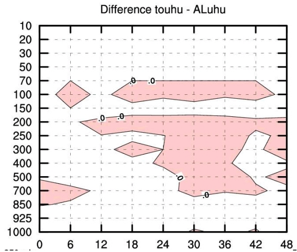
Figure 8: Difference between the root mean square errors of temperature in case of assimilating the humidity data in univariate form: RMSE_{Touhu} - RMSE_{Aluhu} . Negative value (coloured) means that the error of run with ATOVS data is less than that of control run, thus the ATOVS data have positive impact. X and Y axes present the forecast ranges and the model levels respectively.
