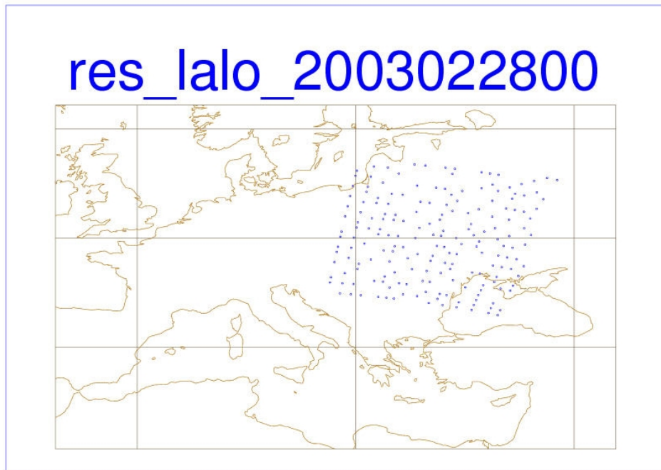
Figure 21: The distribution of the ATOVS pixels at 2003.02.28 00 UTC (situation after screening - active observation).
