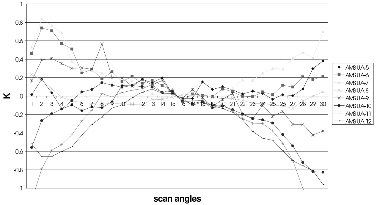
Scan angles bias of AMSUA channels for NOAA-16
